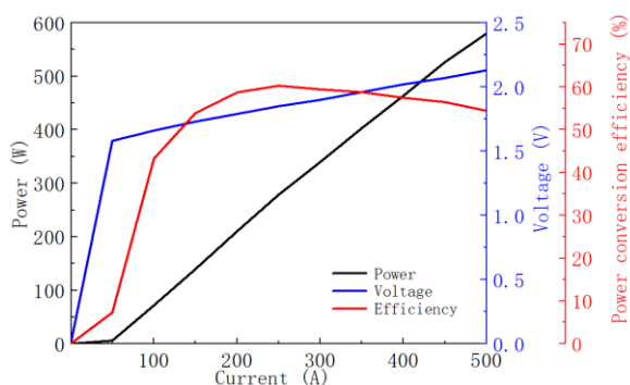
Power-Current-Voltage-Efficiency
